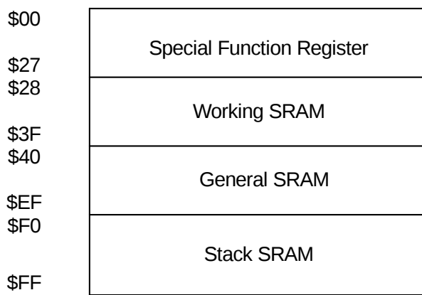
FIGURE 3.3 SRAM Map of AM5BA Series
