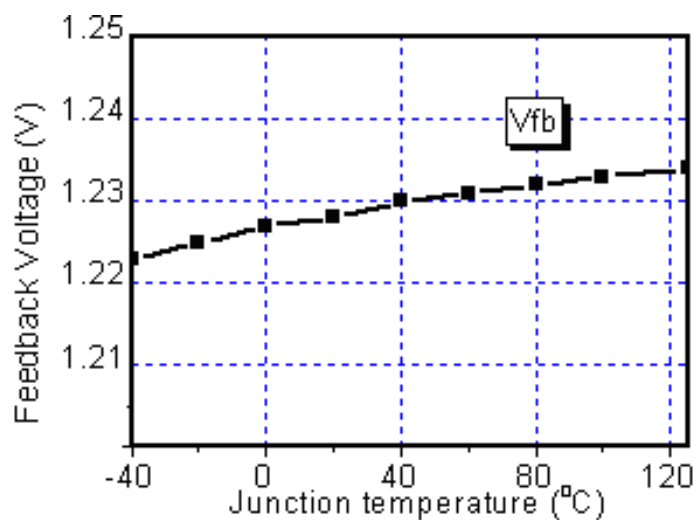
Figure 5. Vfb vs. Temperature
